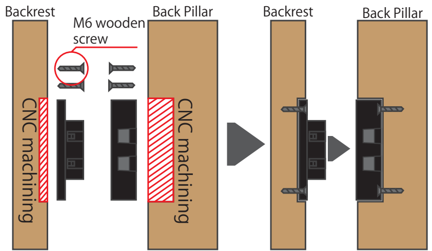
Assembly method
